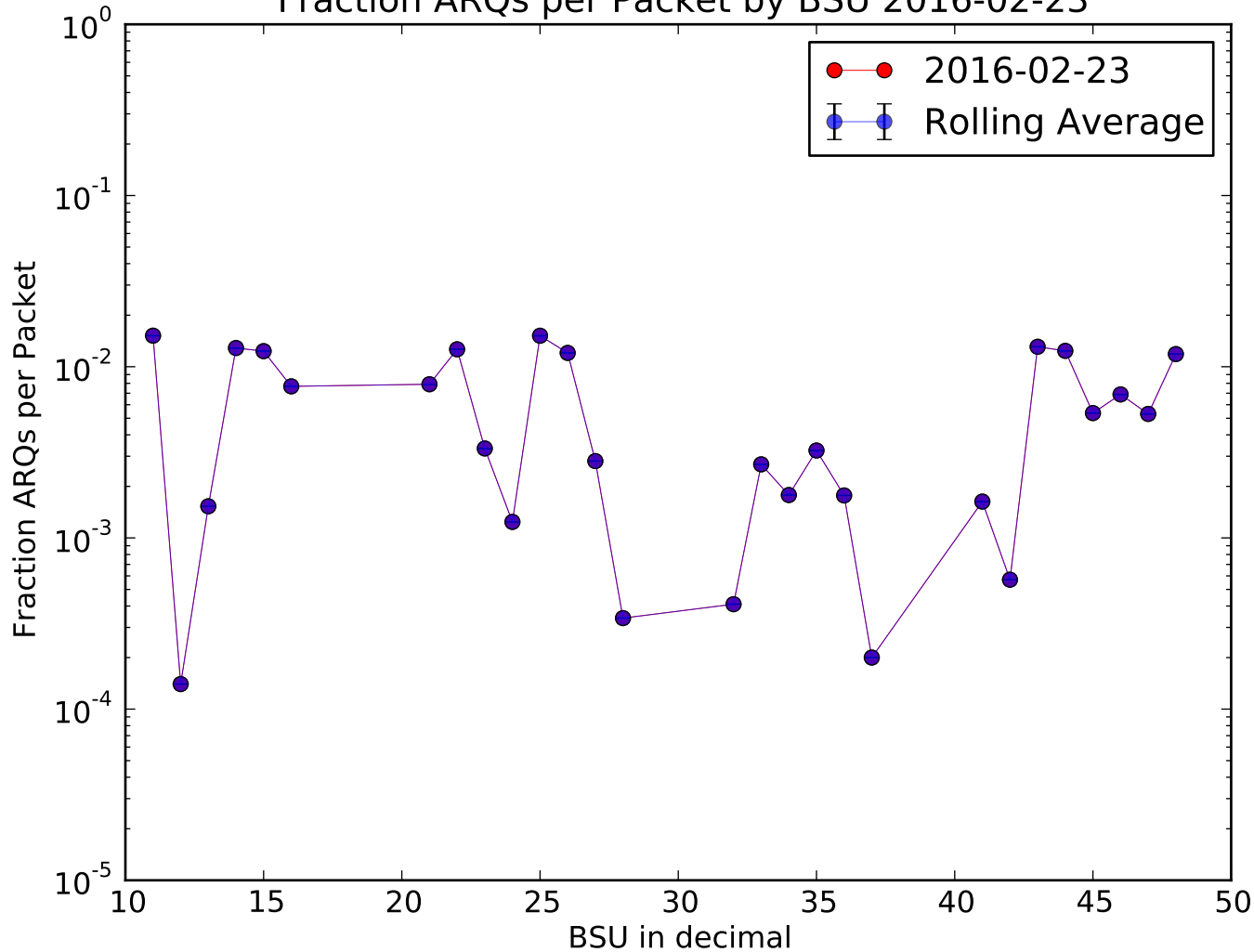
Fraction ARQs per Packet by BSU 2016-02-23
