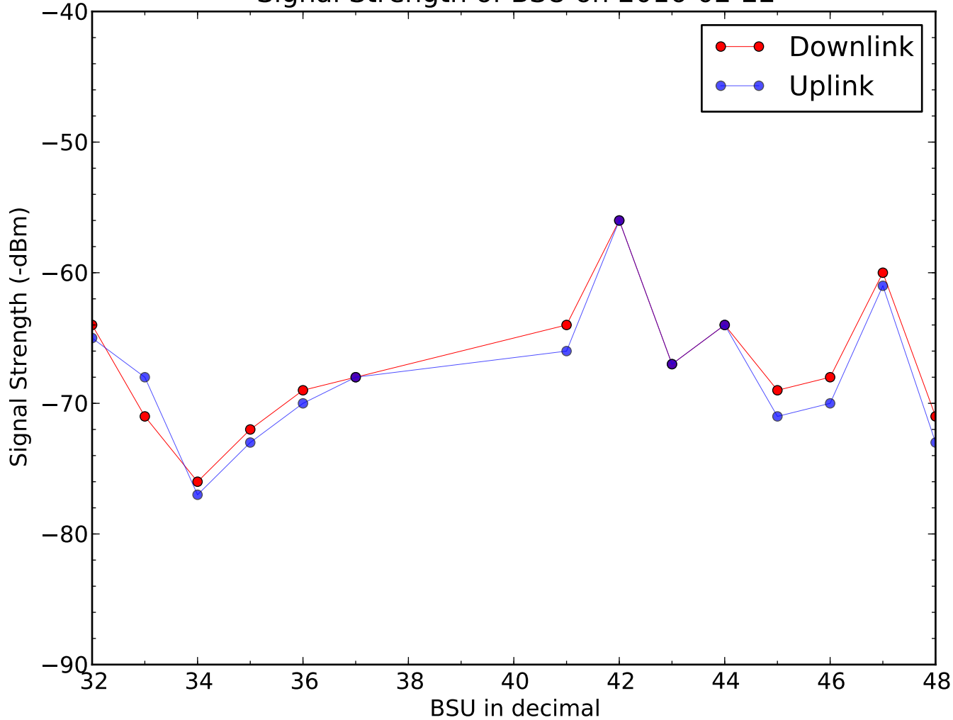
Signal Strength of BSU on 2016-02-22
