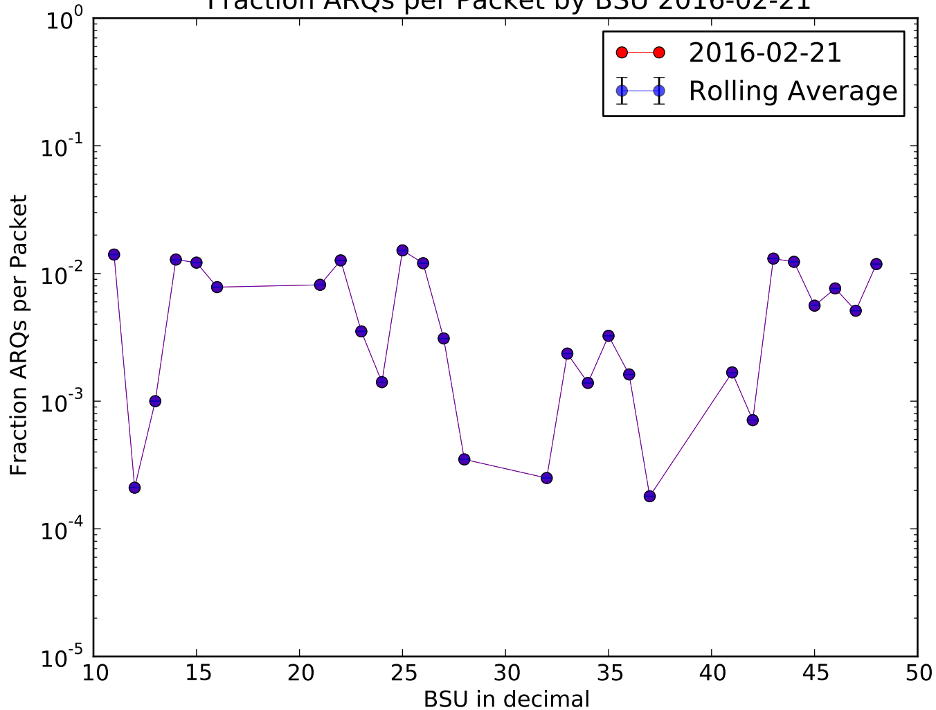
Fraction ARQs per Packet by BSU 2016-02-21
