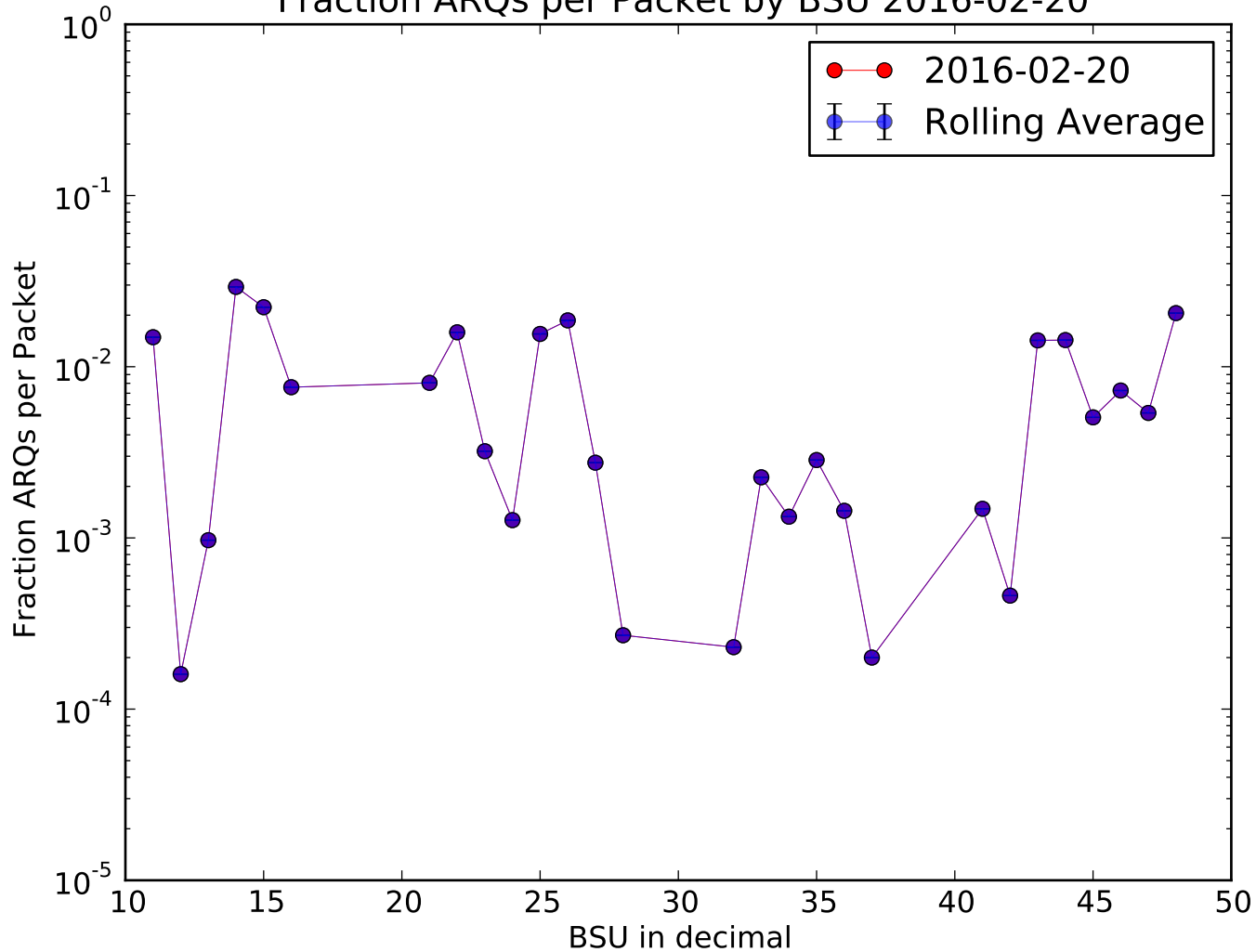
Fraction ARQs per Packet by BSU 2016-02-20
