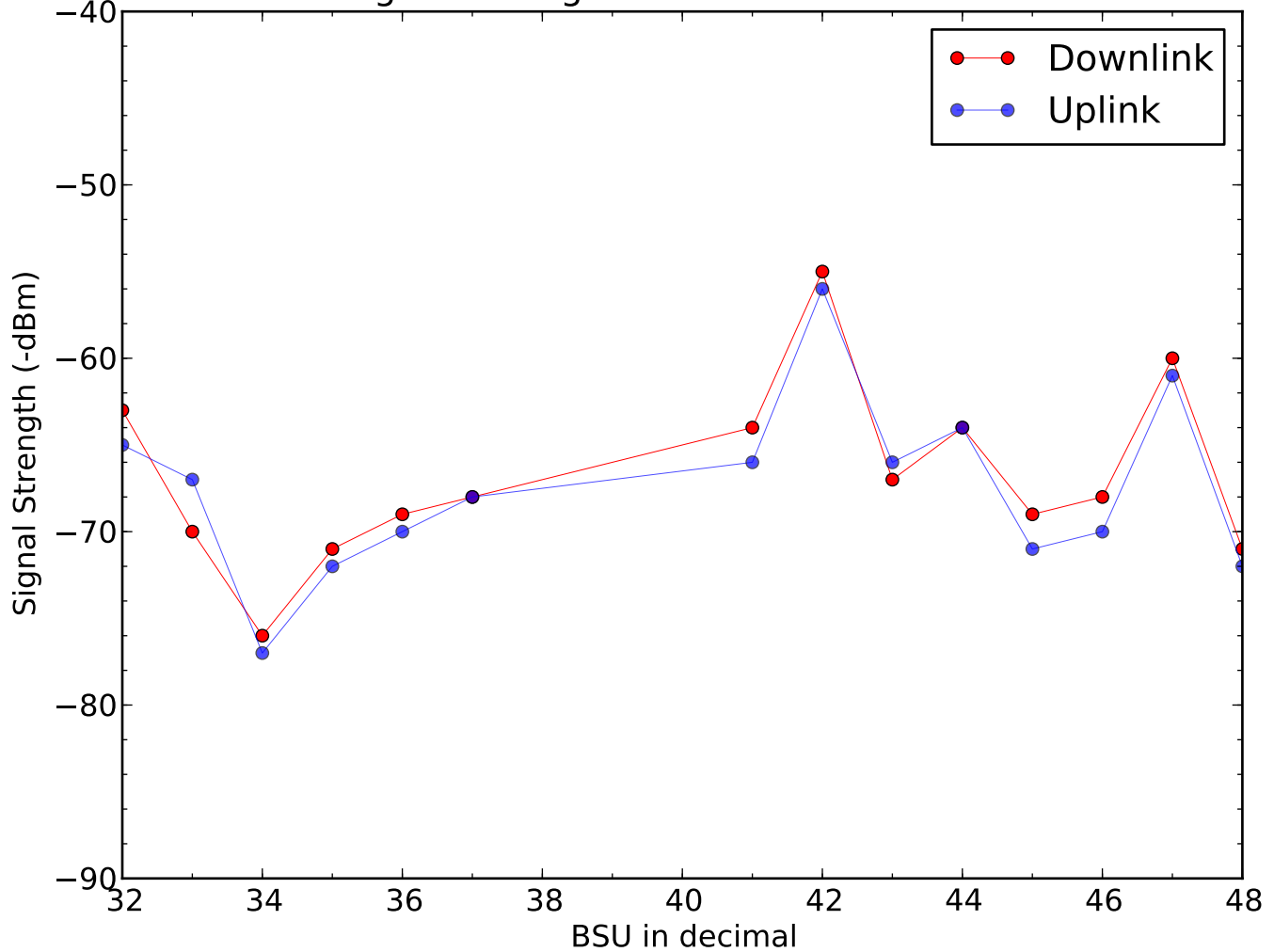
Signal Strength of BSU on 2016-02-15
