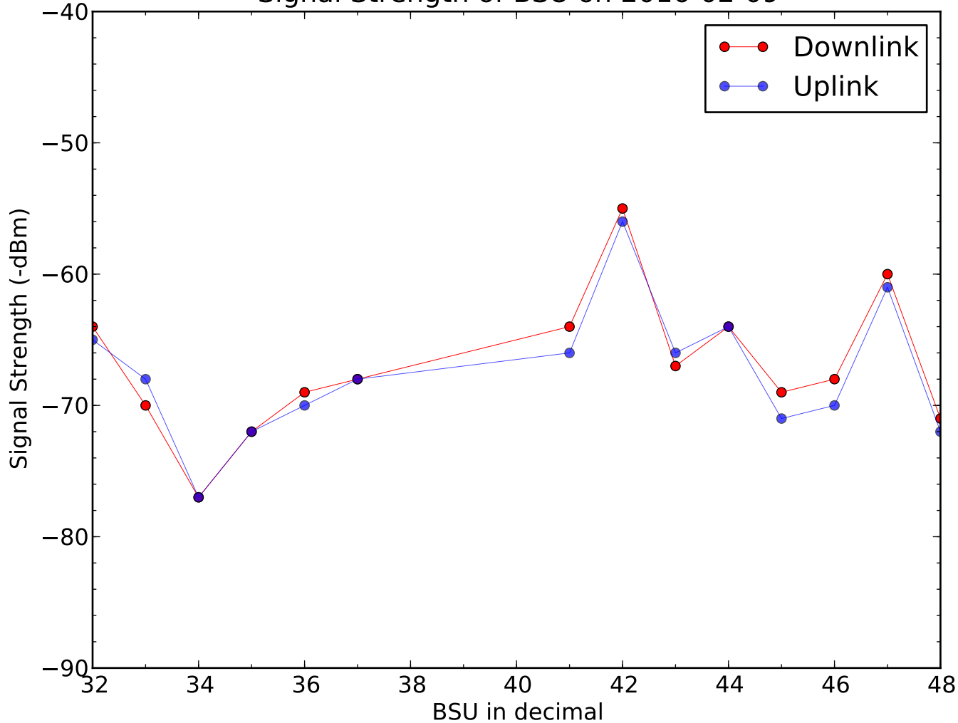
Signal Strength of BSU on 2016-02-09
