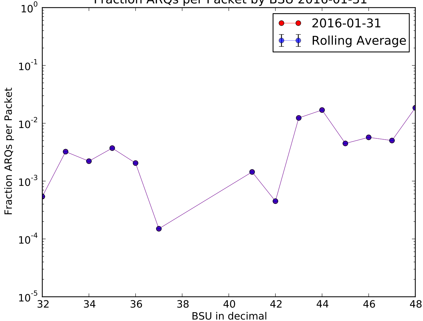
Fraction ARQs per Packet by BSU 2016-01-31
