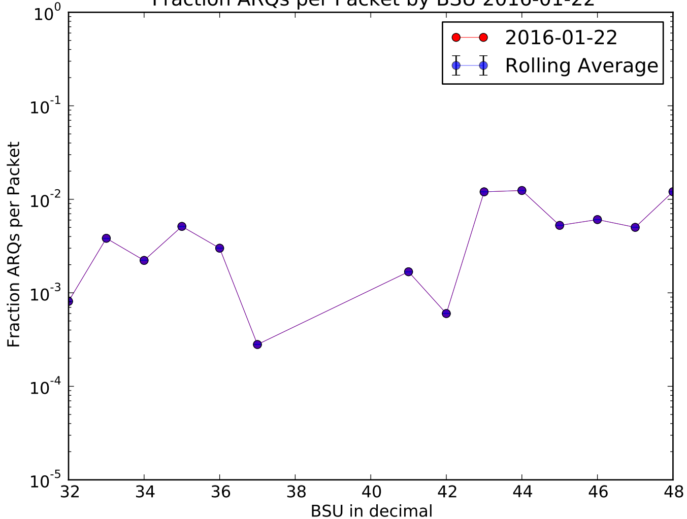
Fraction ARQs per Packet by BSU 2016-01-22
