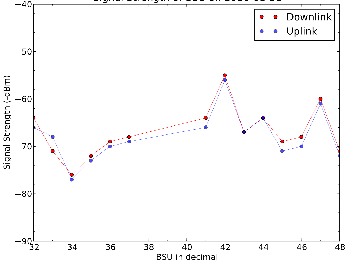
Signal Strength of BSU on 2016-01-21
