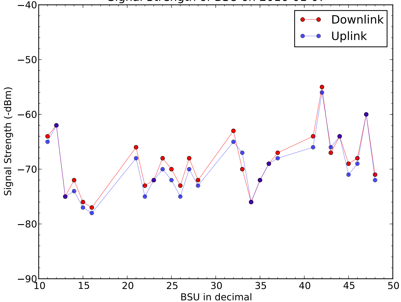
Signal Strength of BSU on 2016-01-07
