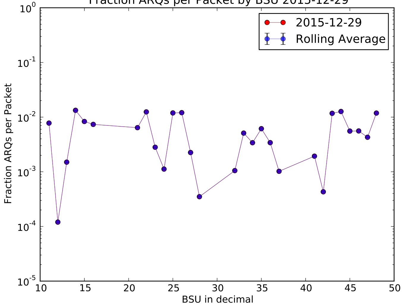
Fraction ARQs per Packet by BSU 2015-12-29
