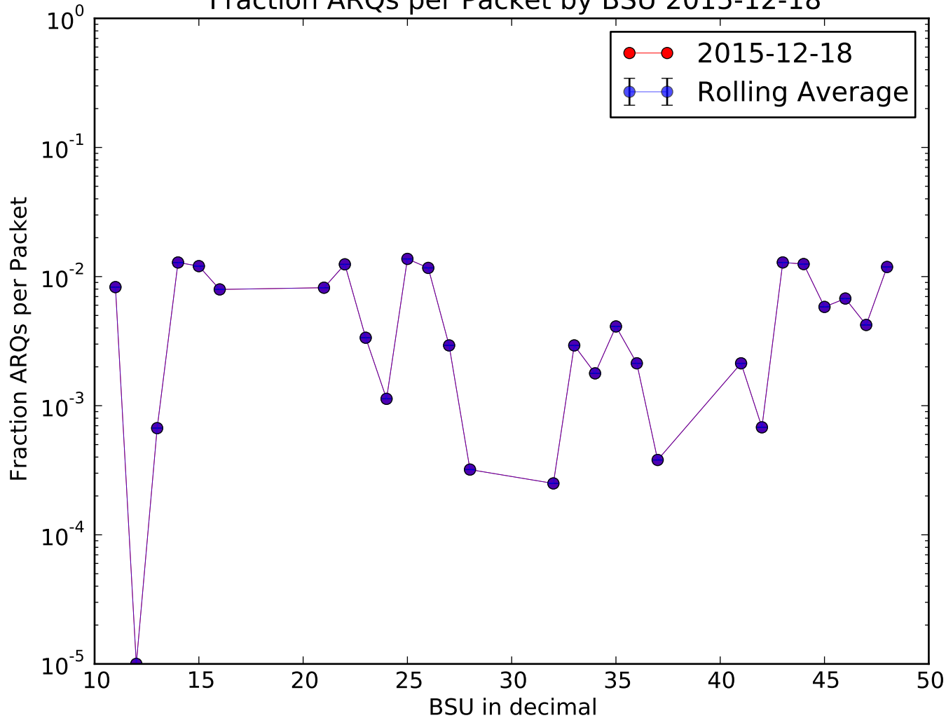
Fraction ARQs per Packet by BSU 2015-12-18
