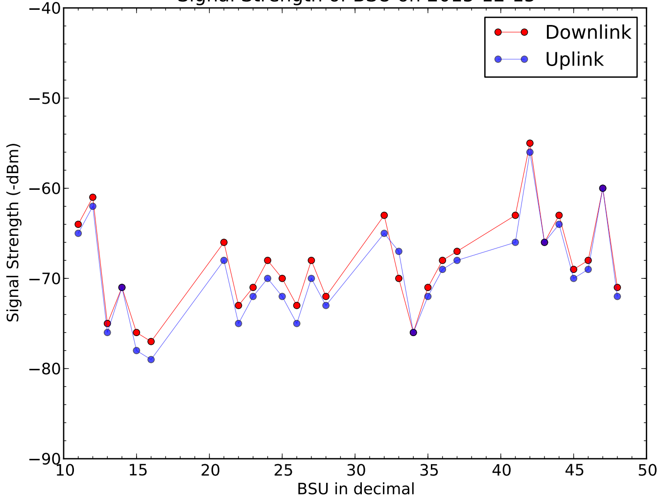
Signal Strength of BSU on 2015-12-15
