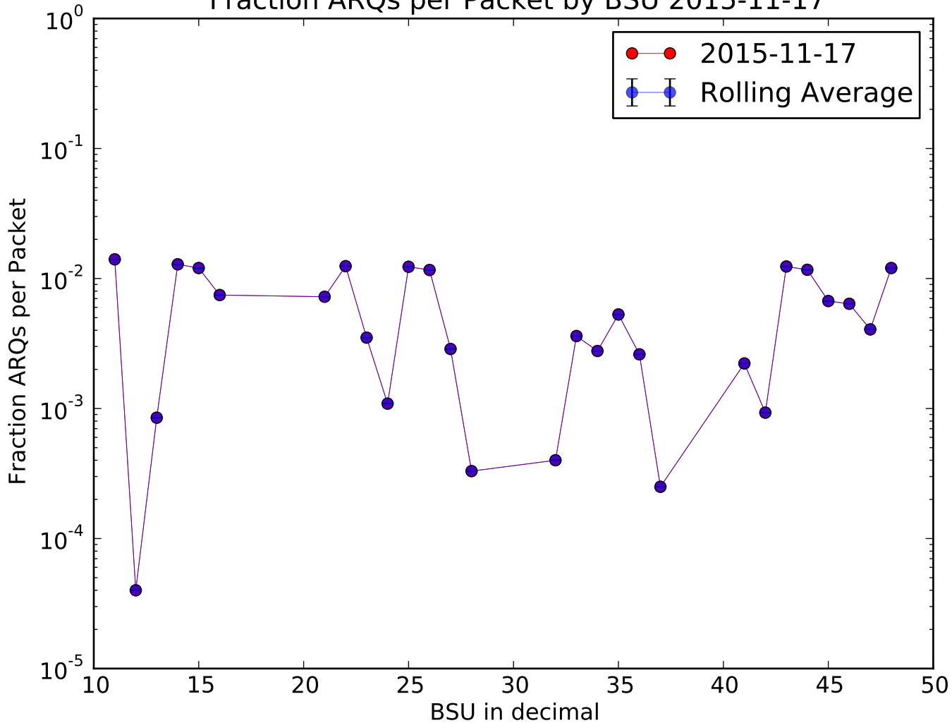
Fraction ARQs per Packet by BSU 2015-11-17
