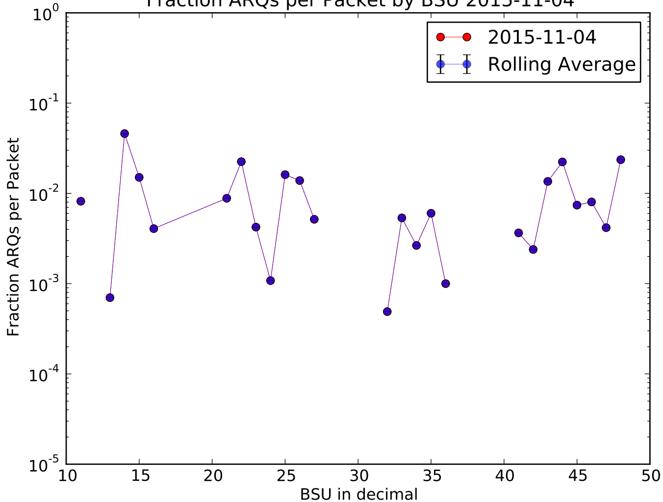
Fraction ARQs per Packet by BSU 2015-11-04
