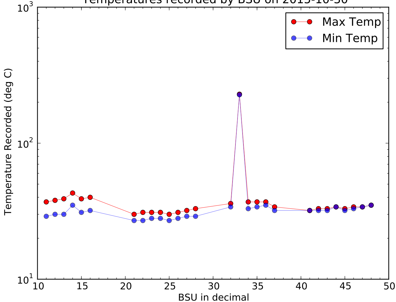
Temperatures recorded by BSU on 2015-10-30
