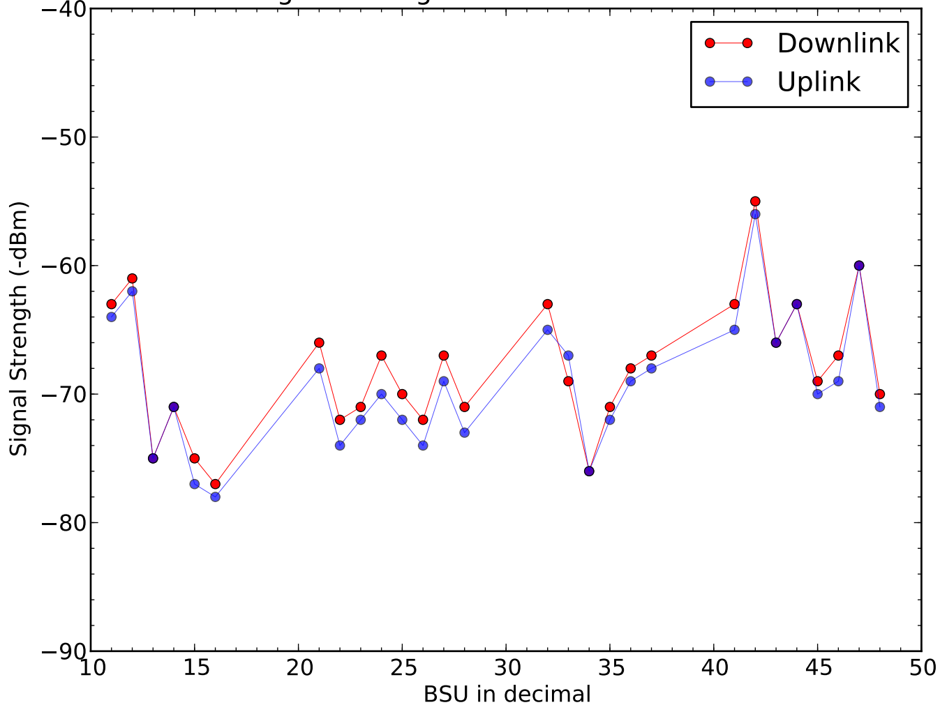
Signal Strength of BSU on 2015-10-30
