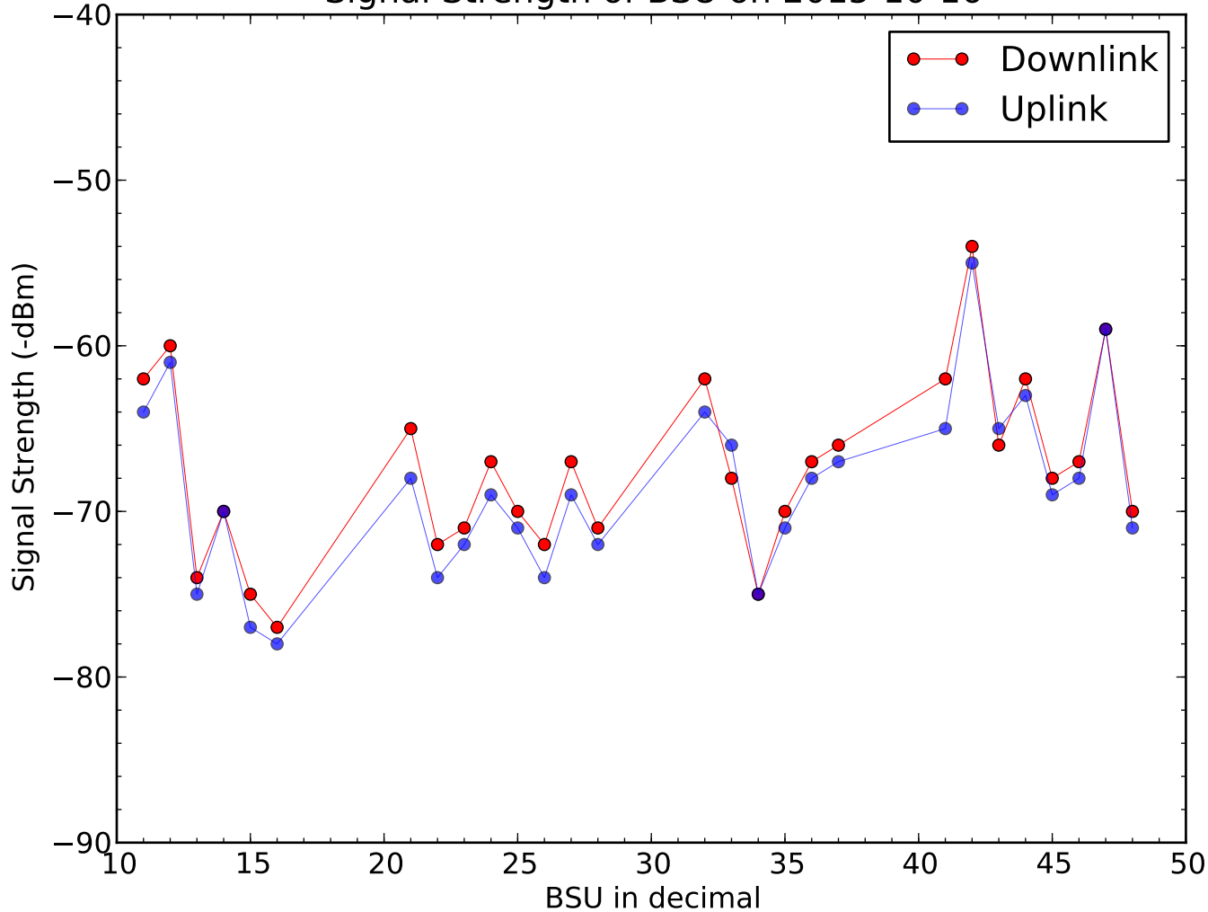
Signal Strength of BSU on 2015-10-16
