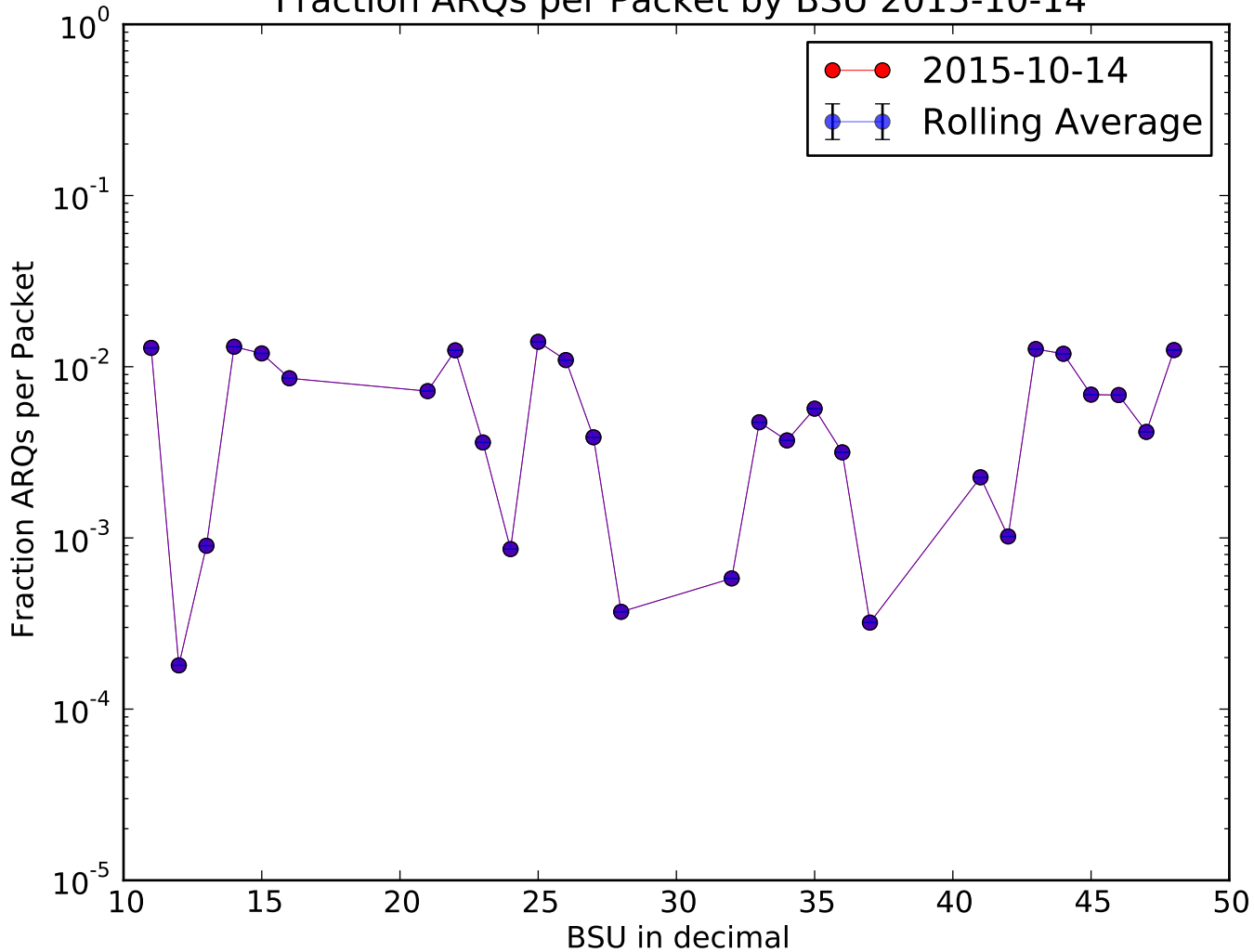
Fraction ARQs per Packet by BSU 2015-10-14
