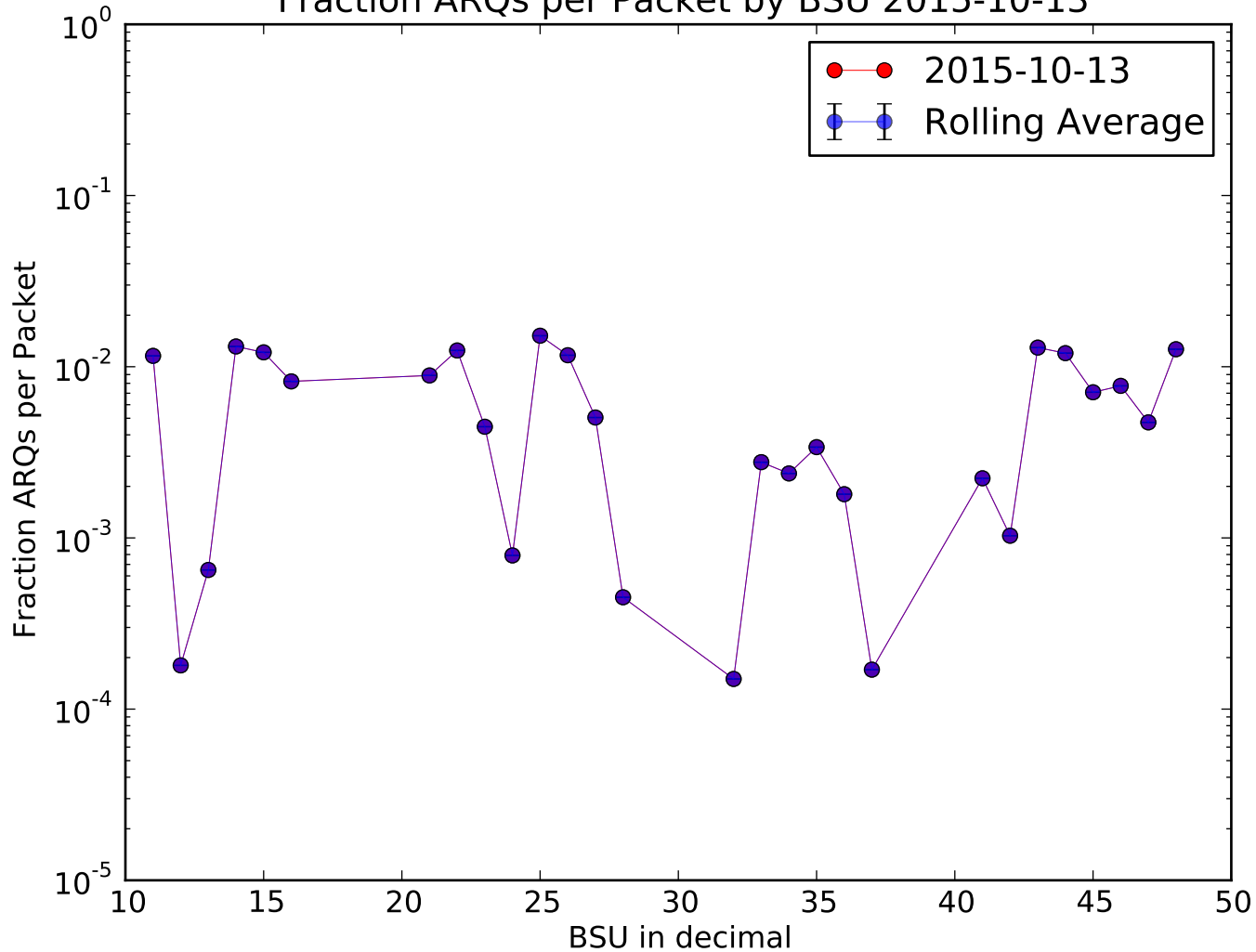
Fraction ARQs per Packet by BSU 2015-10-13
