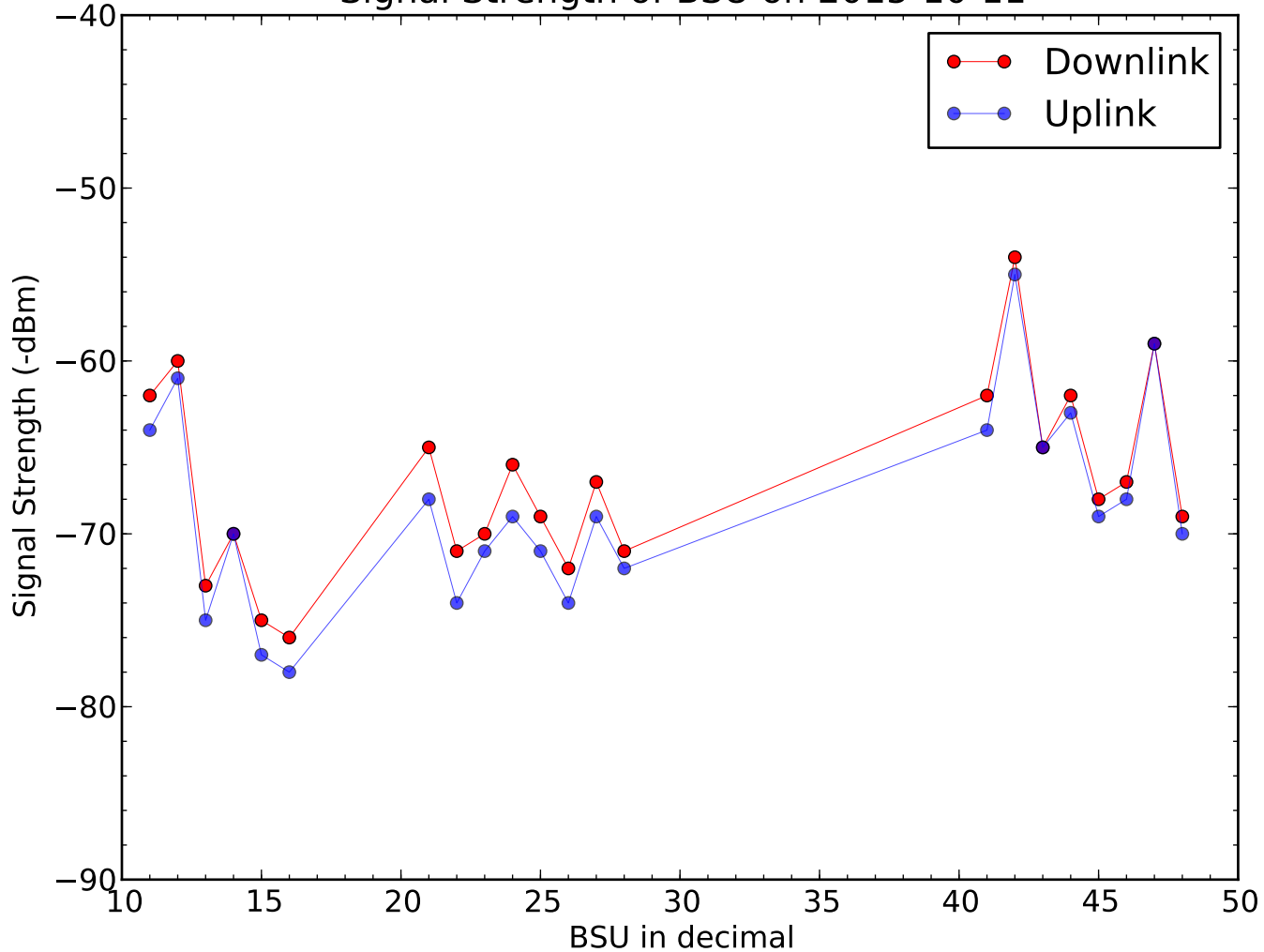
Signal Strength of BSU on 2015-10-11
