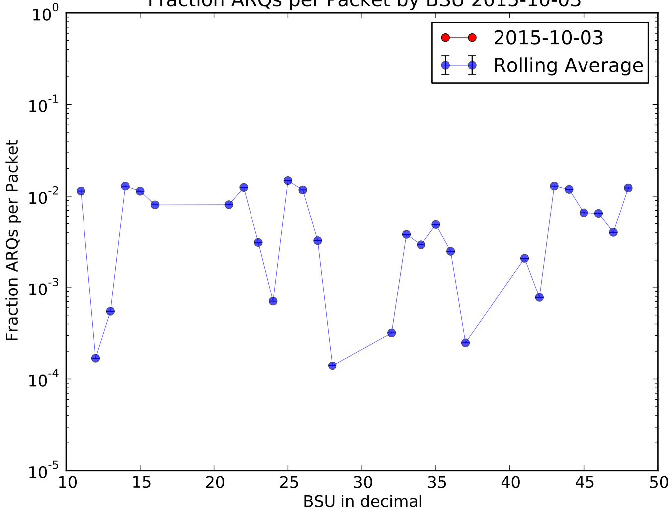
Fraction ARQs per Packet by BSU 2015-10-03
