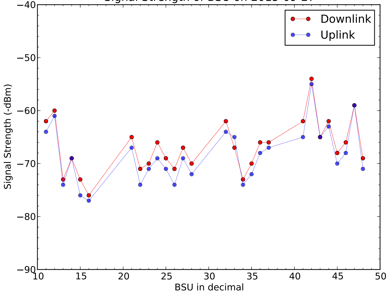
Signal Strength of BSU on 2015-09-27
