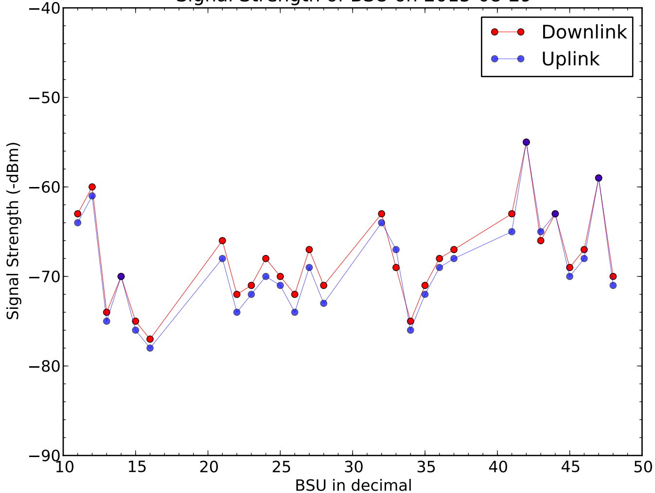
Signal Strength of BSU on 2015-08-29
