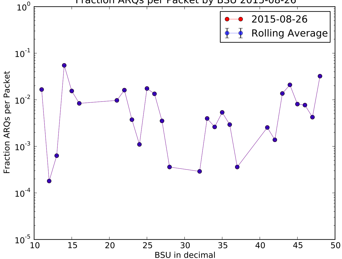
Fraction ARQs per Packet by BSU 2015-08-26
