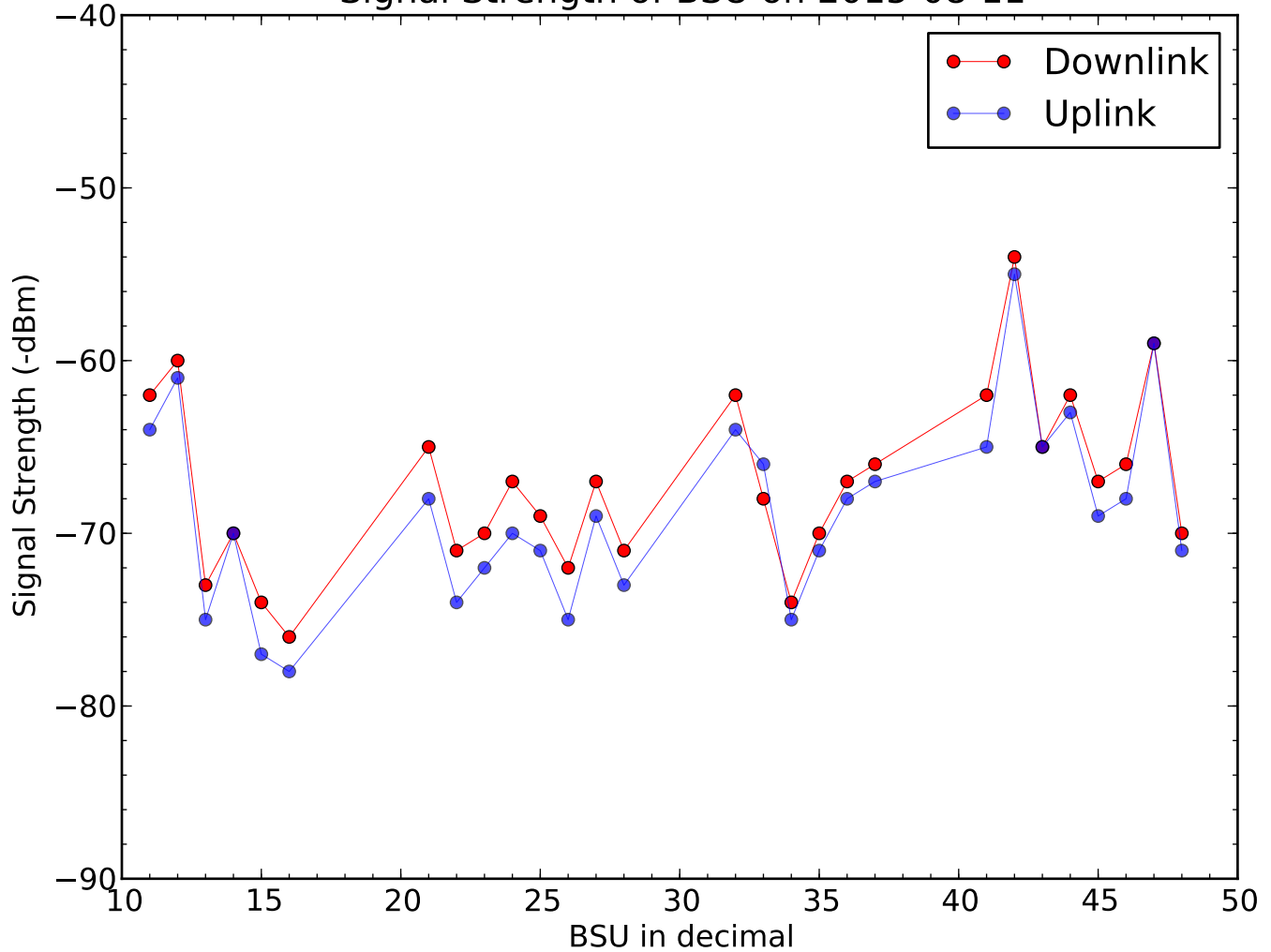
Signal Strength of BSU on 2015-08-11
