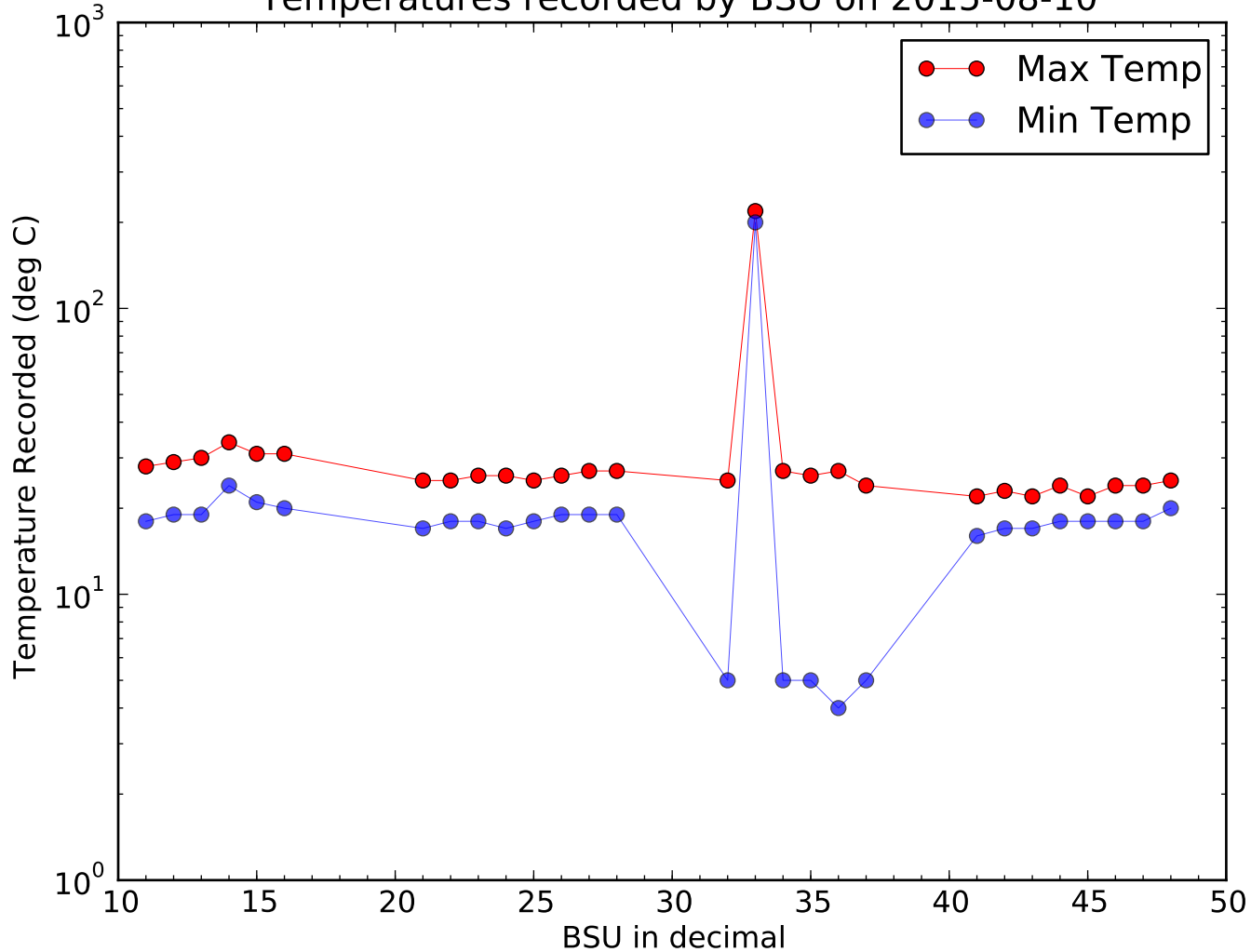
Temperatures recorded by BSU on 2015-08-10
