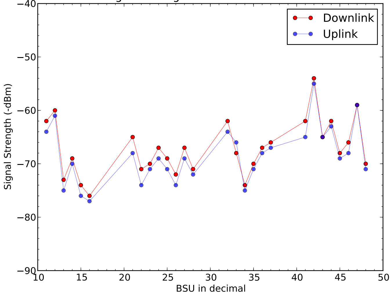
Signal Strength of BSU on 2015-08-01
