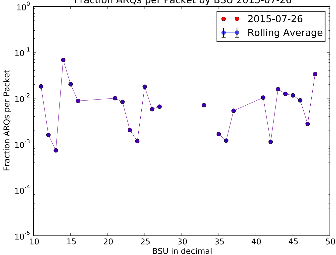
Fraction ARQs per Packet by BSU 2015-07-26
