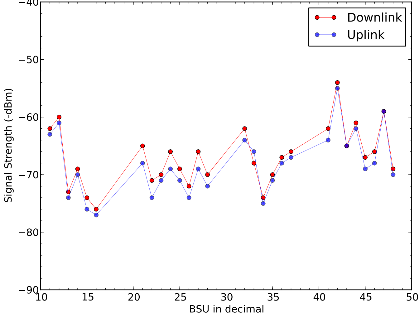
Signal Strength of BSU on 2015-07-18
