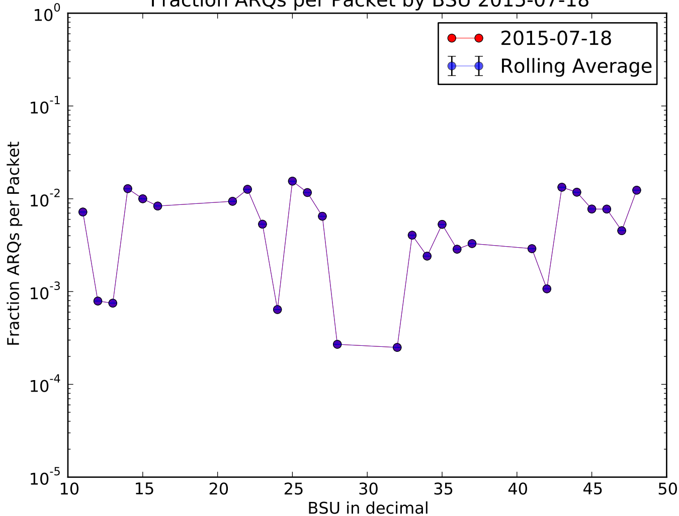
Fraction ARQs per Packet by BSU 2015-07-18
