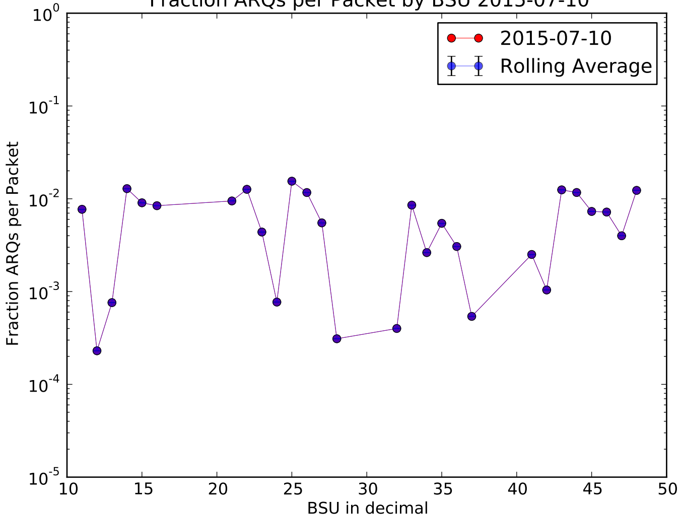
Fraction ARQs per Packet by BSU 2015-07-10
