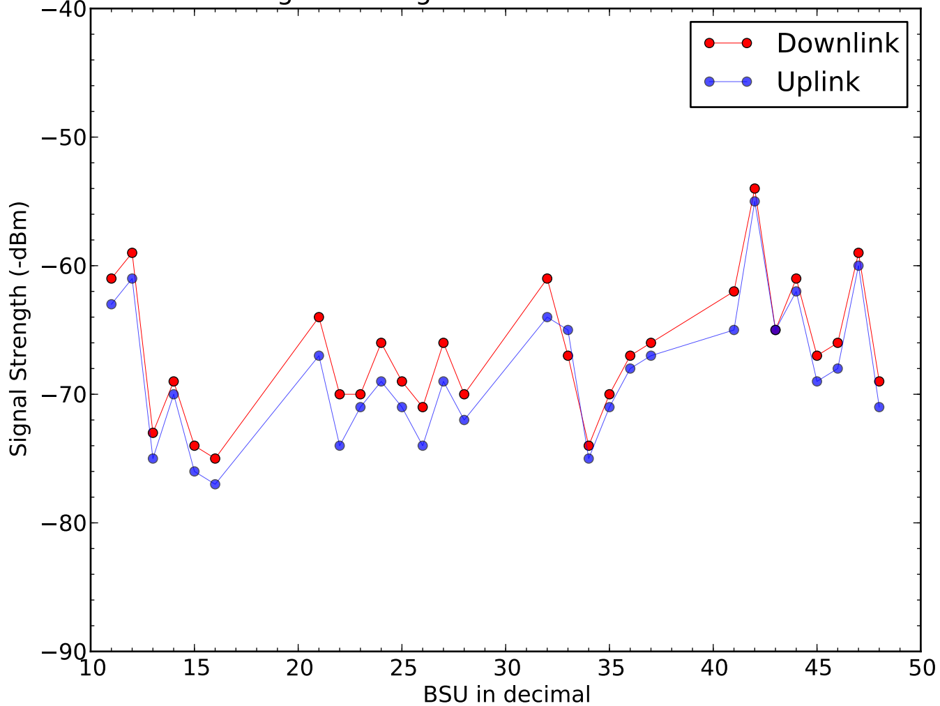
Signal Strength of BSU on 2015-06-29
