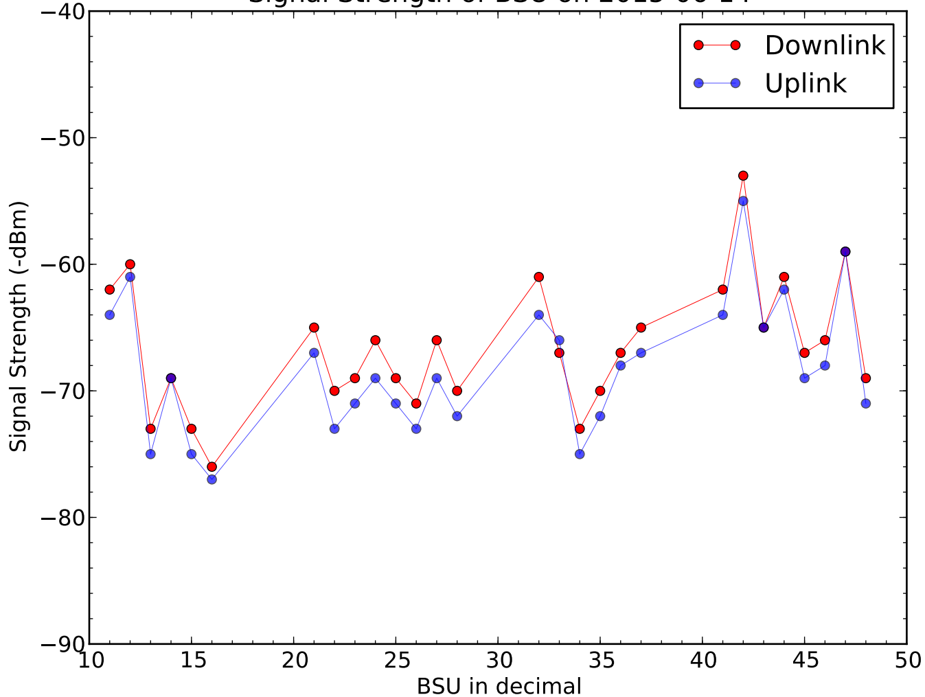
Signal Strength of BSU on 2015-06-14
