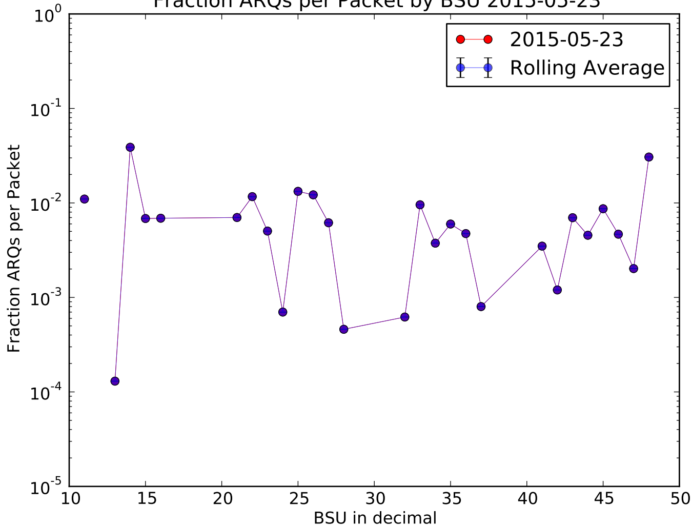
Fraction ARQs per Packet by BSU 2015-05-23
