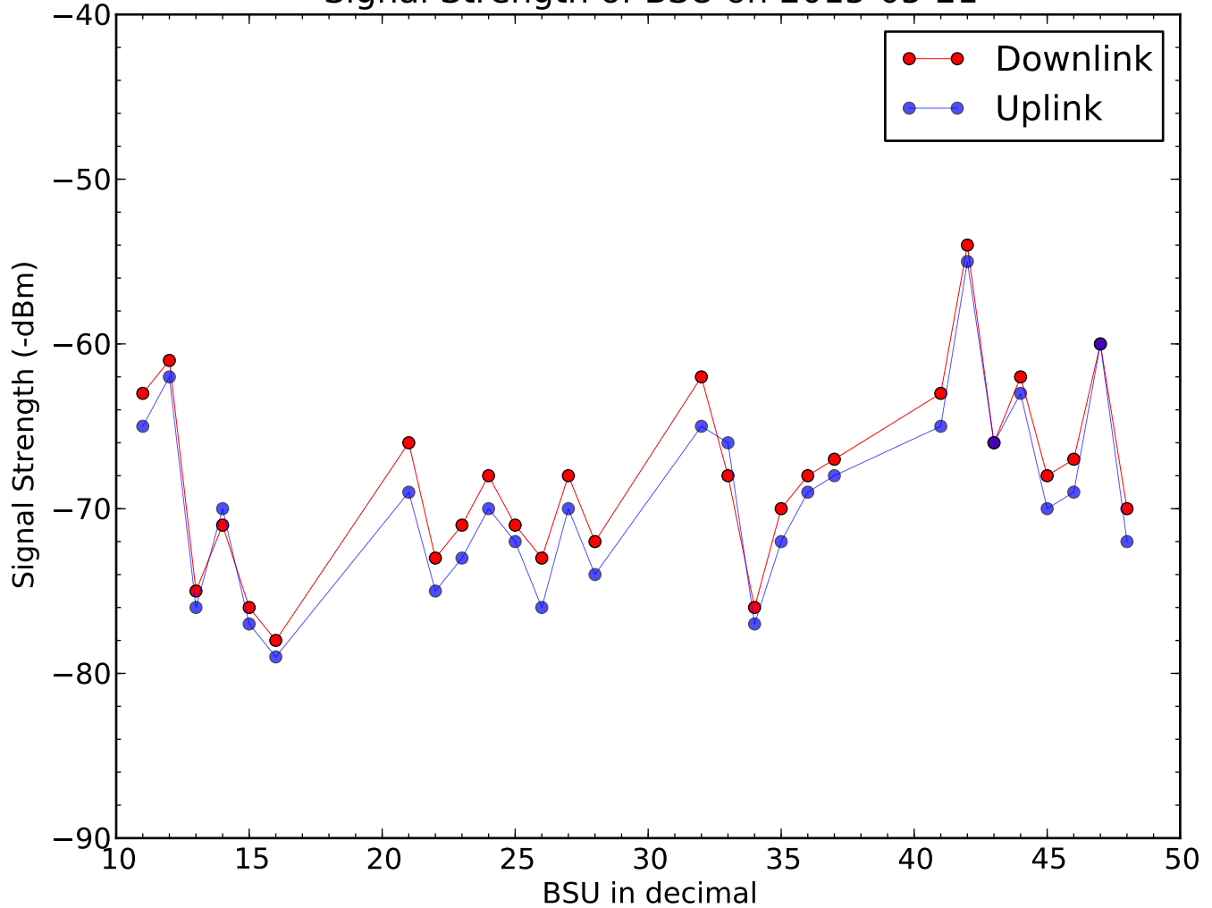
Signal Strength of BSU on 2015-05-21
