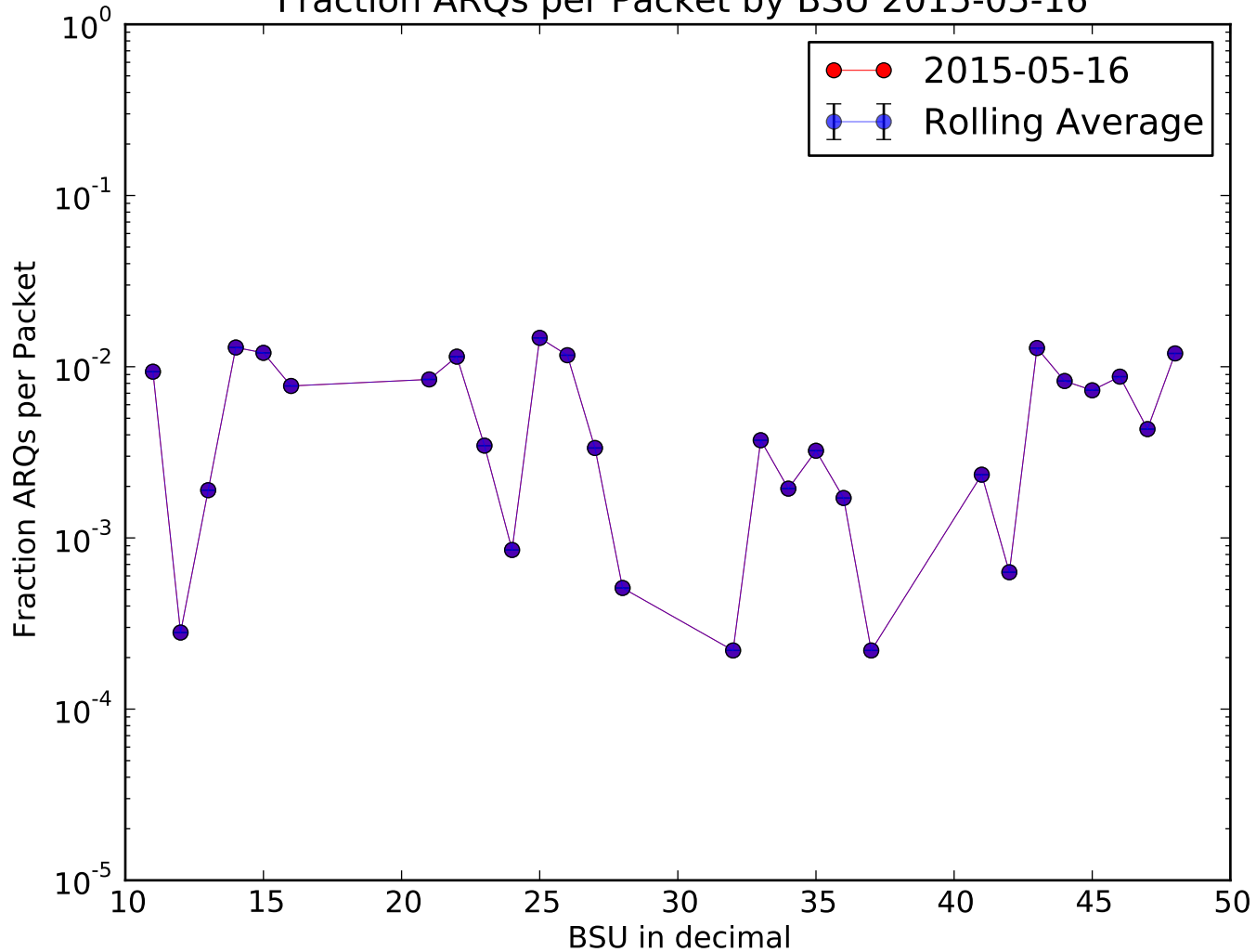
Fraction ARQs per Packet by BSU 2015-05-16
