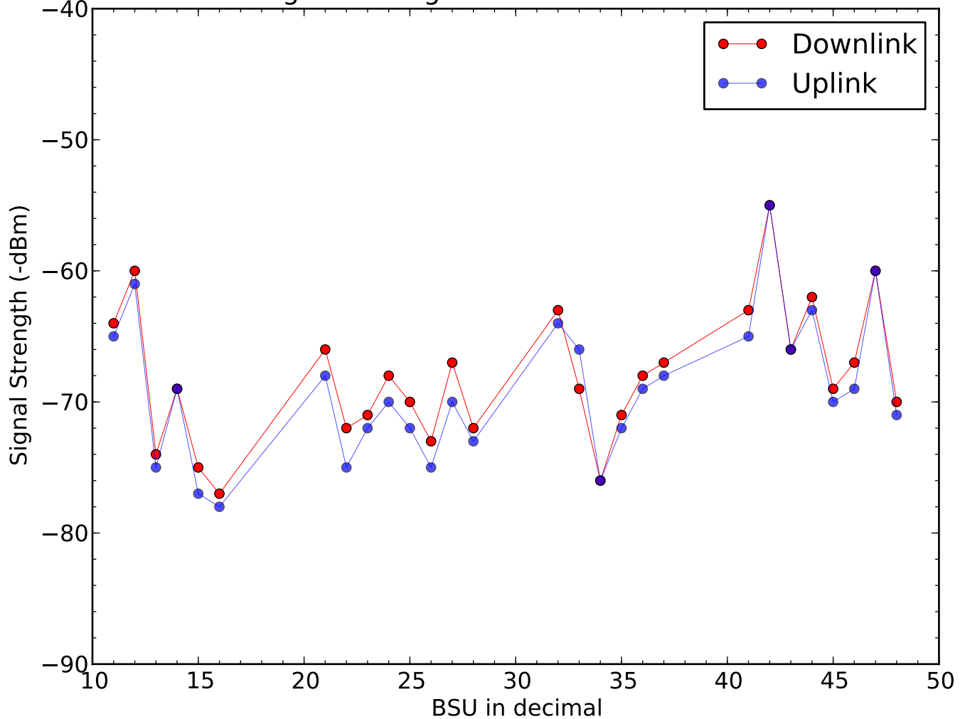
Signal Strength of BSU on 2015-05-13
