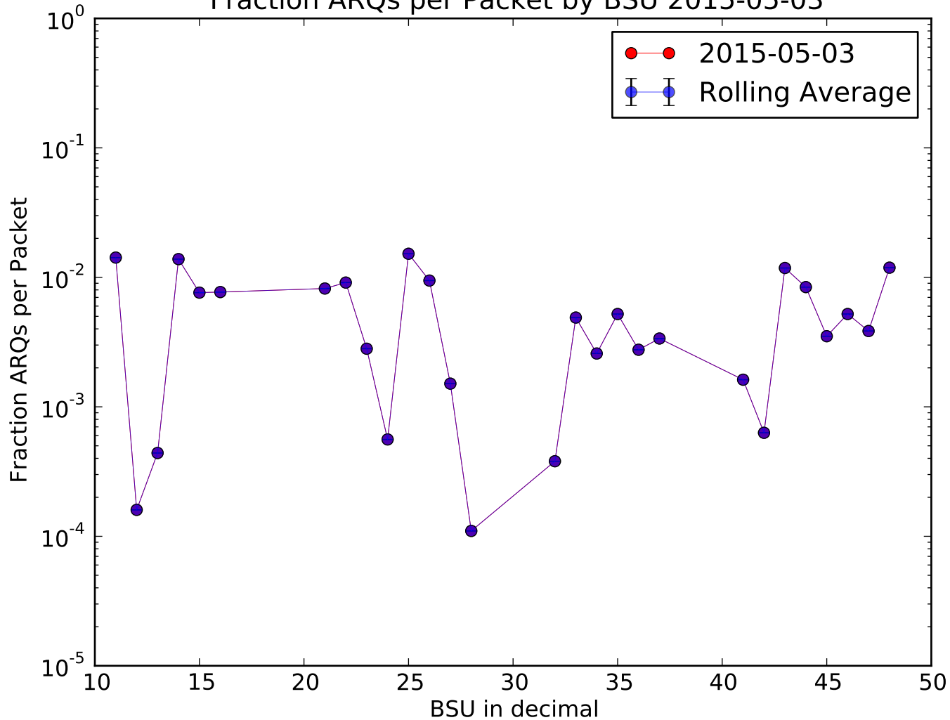
Fraction ARQs per Packet by BSU 2015-05-03
