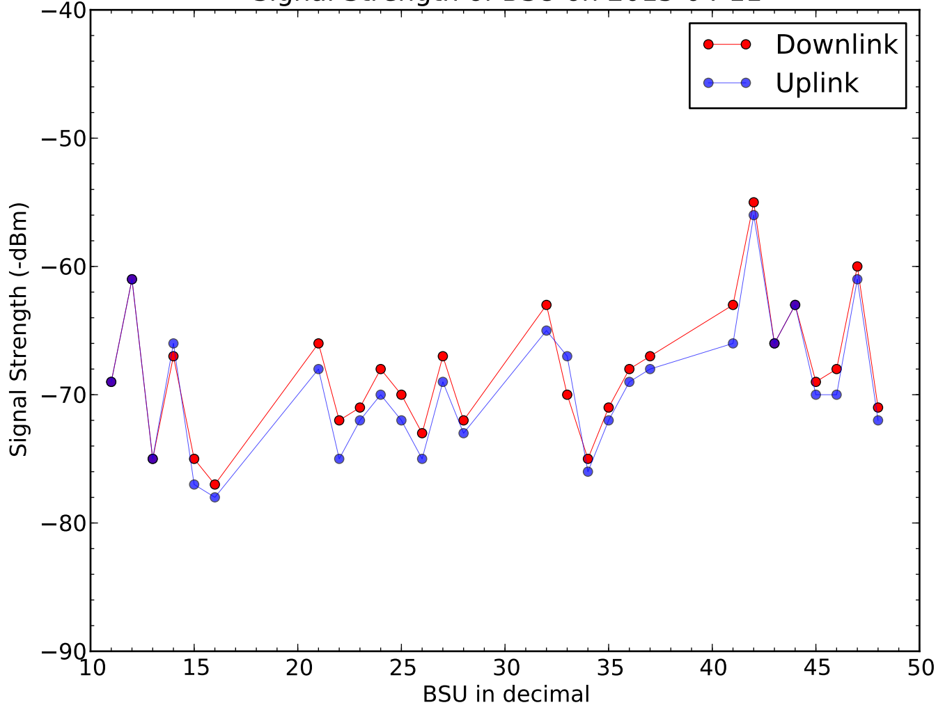
Signal Strength of BSU on 2015-04-11
