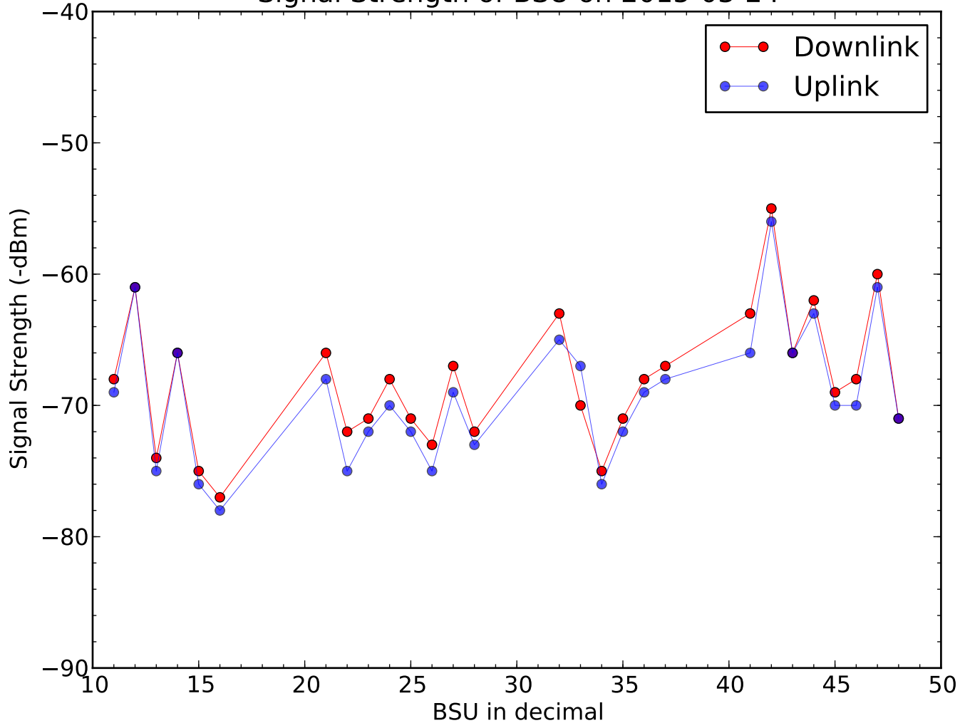
Signal Strength of BSU on 2015-03-24
