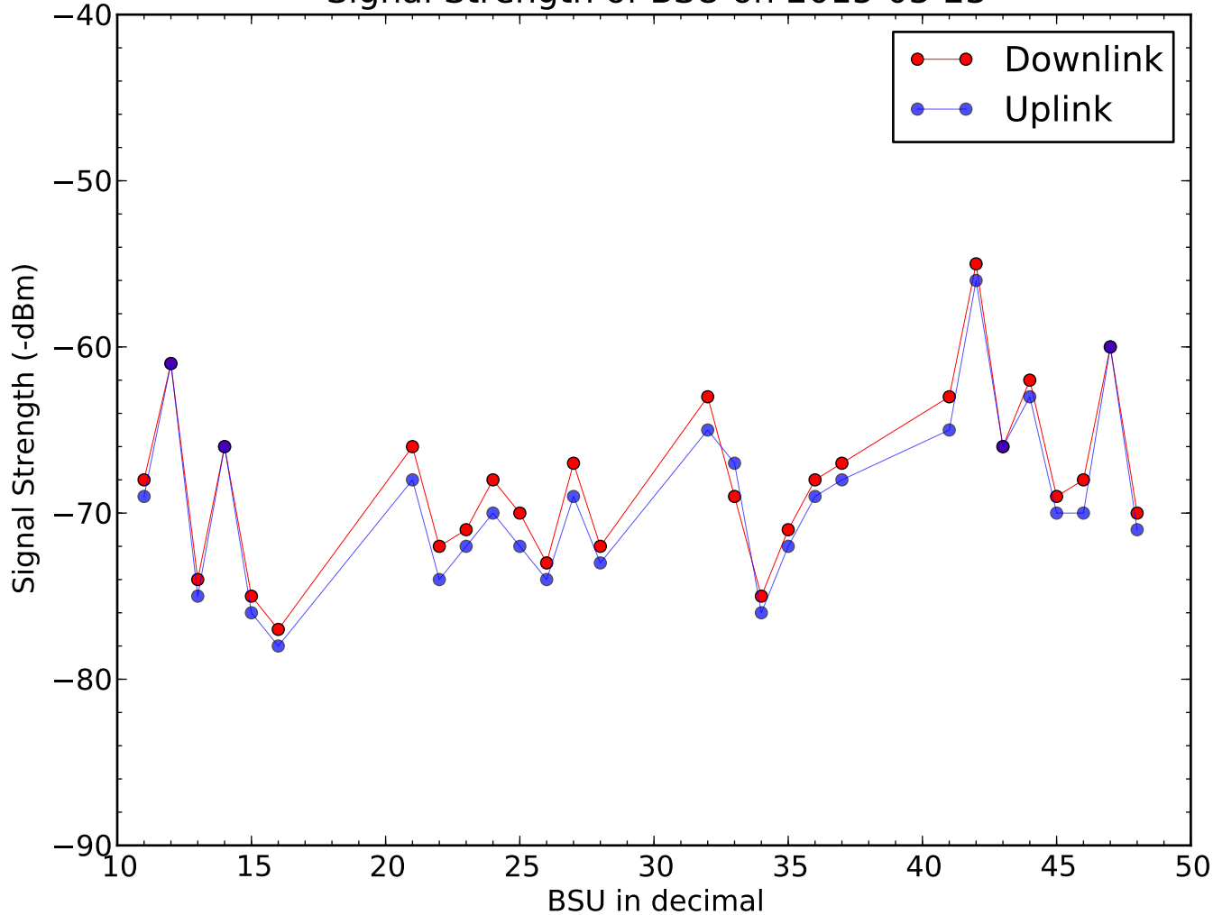
Signal Strength of BSU on 2015-03-23
