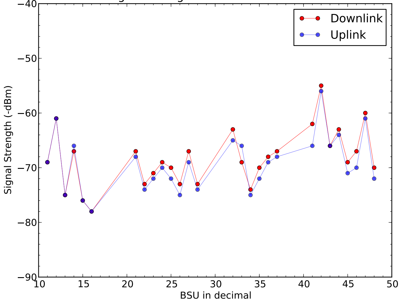
Signal Strength of BSU on 2015-03-17
