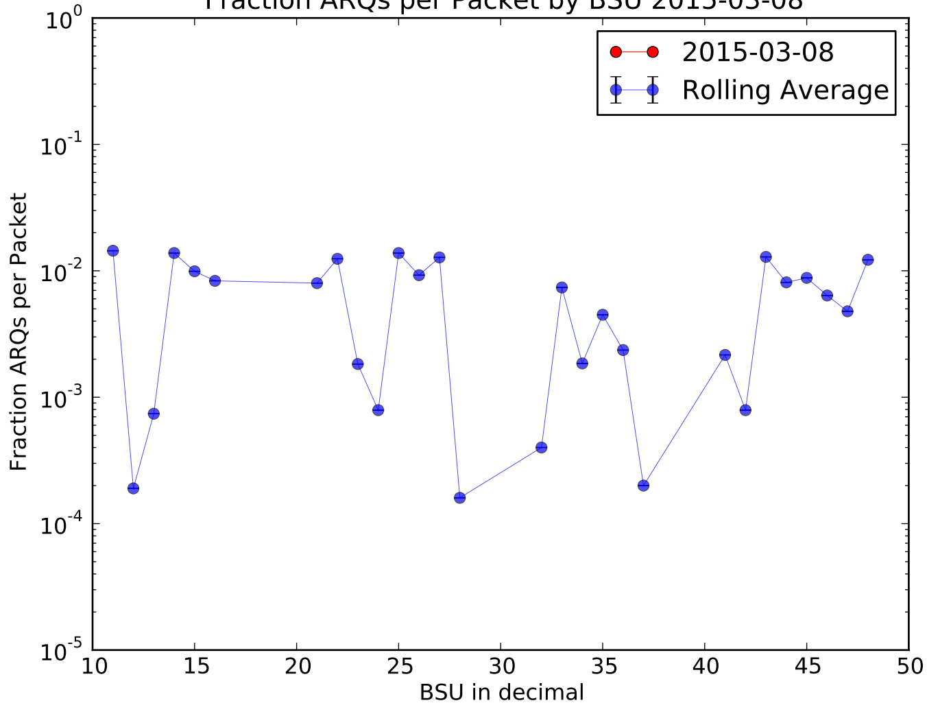
Fraction ARQs per Packet by BSU 2015-03-08
