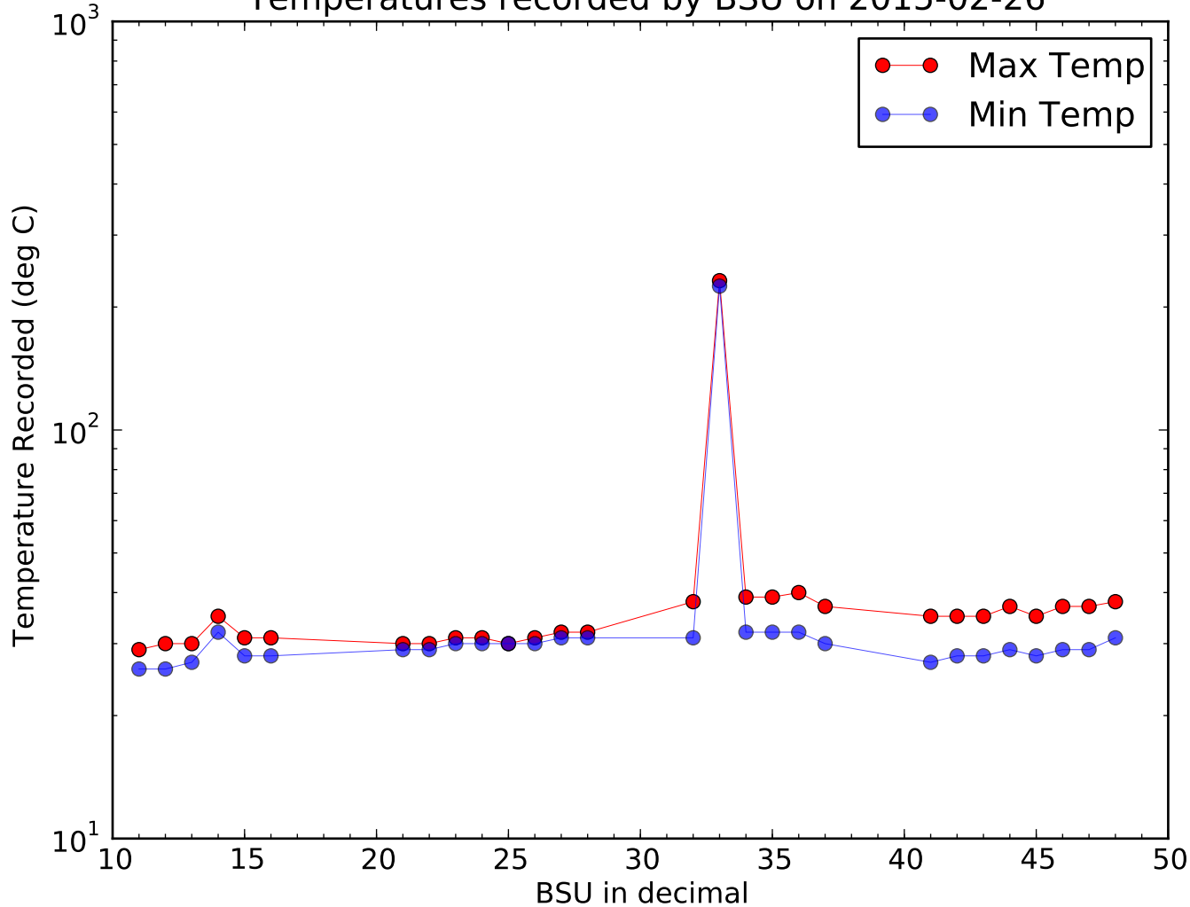
Temperatures recorded by BSU on 2015-02-26
