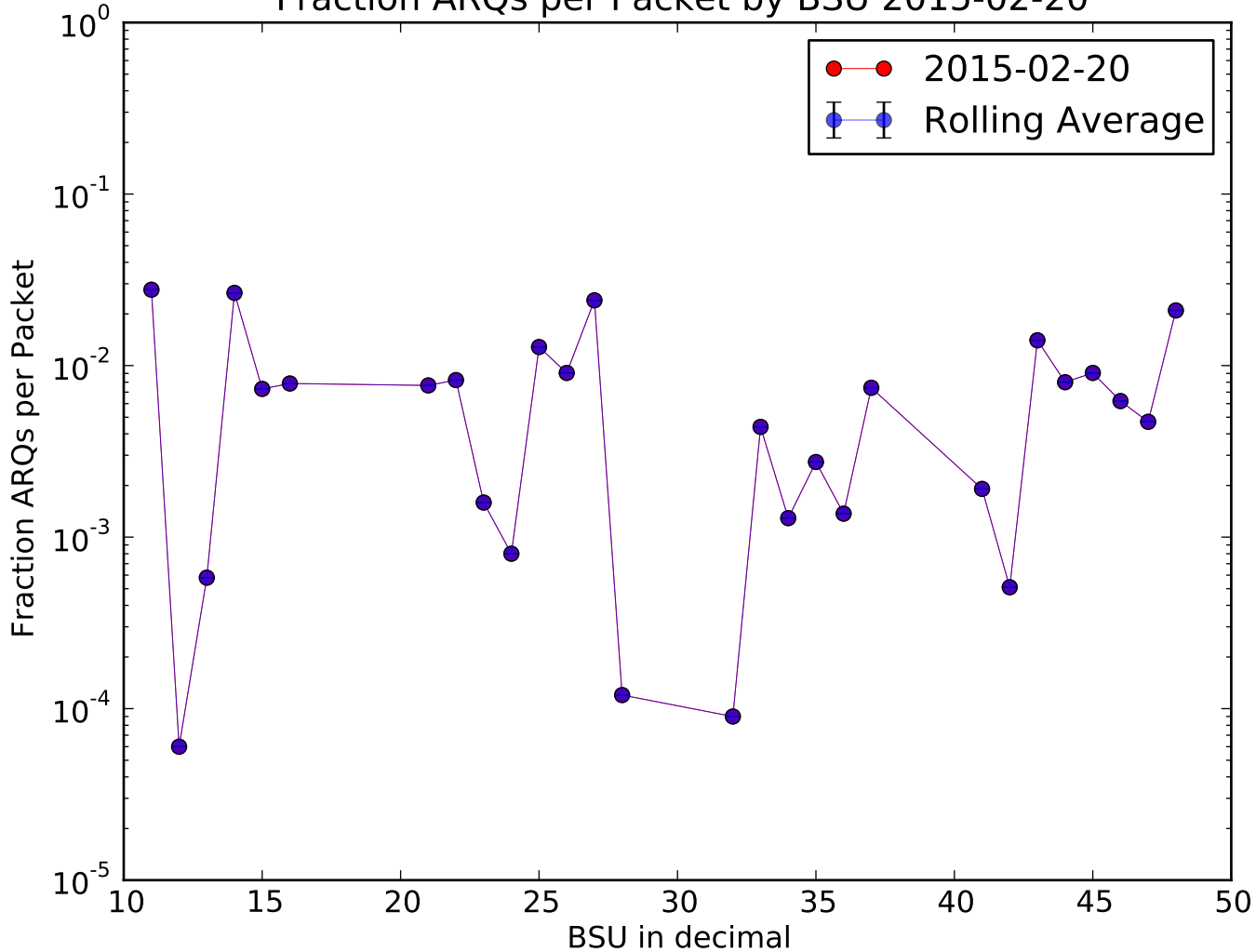
Fraction ARQs per Packet by BSU 2015-02-20
