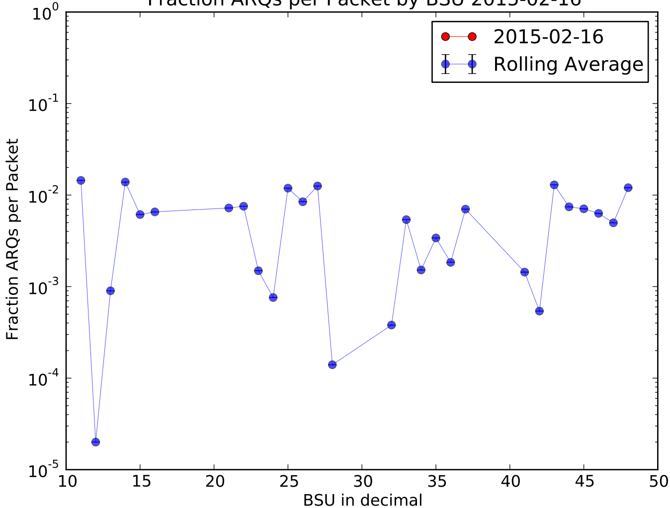
Fraction ARQs per Packet by BSU 2015-02-16
