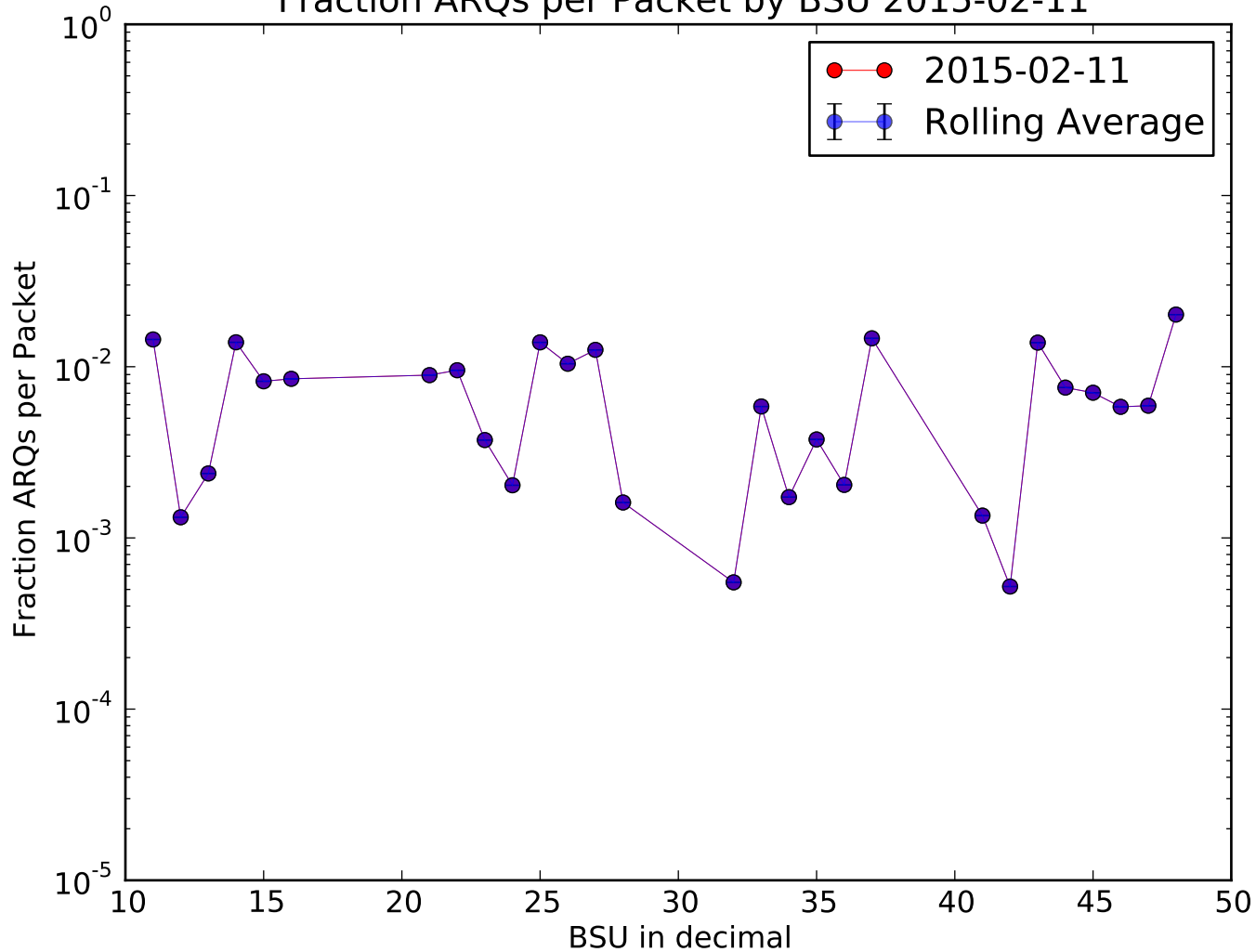
Fraction ARQs per Packet by BSU 2015-02-11
