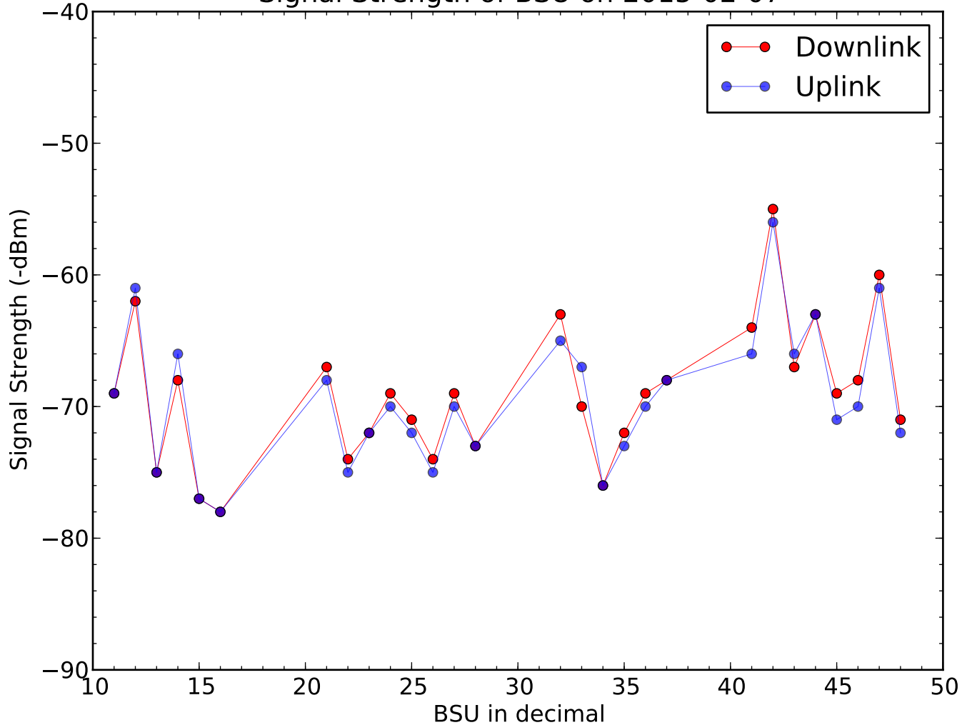
Signal Strength of BSU on 2015-02-07
