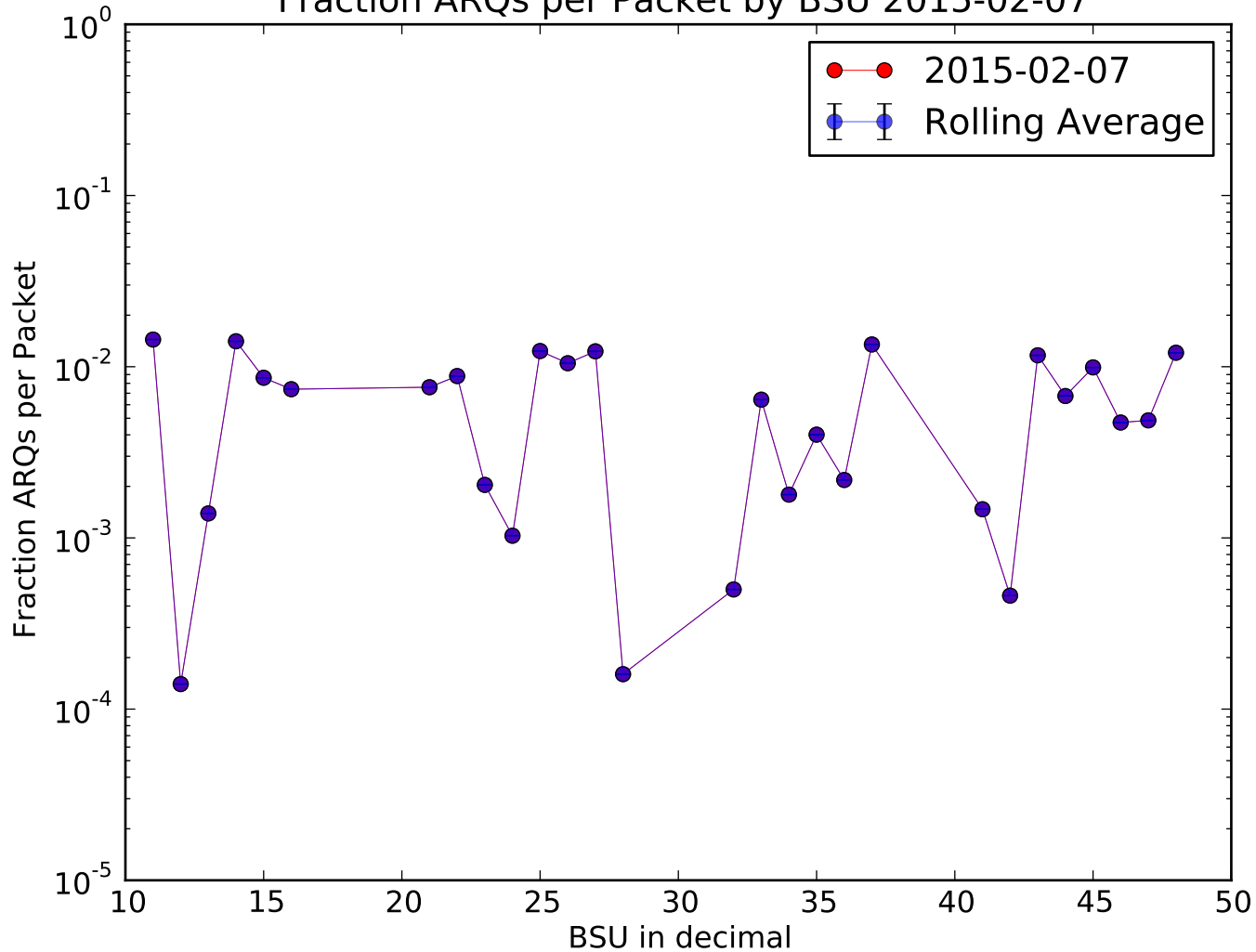
Fraction ARQs per Packet by BSU 2015-02-07
